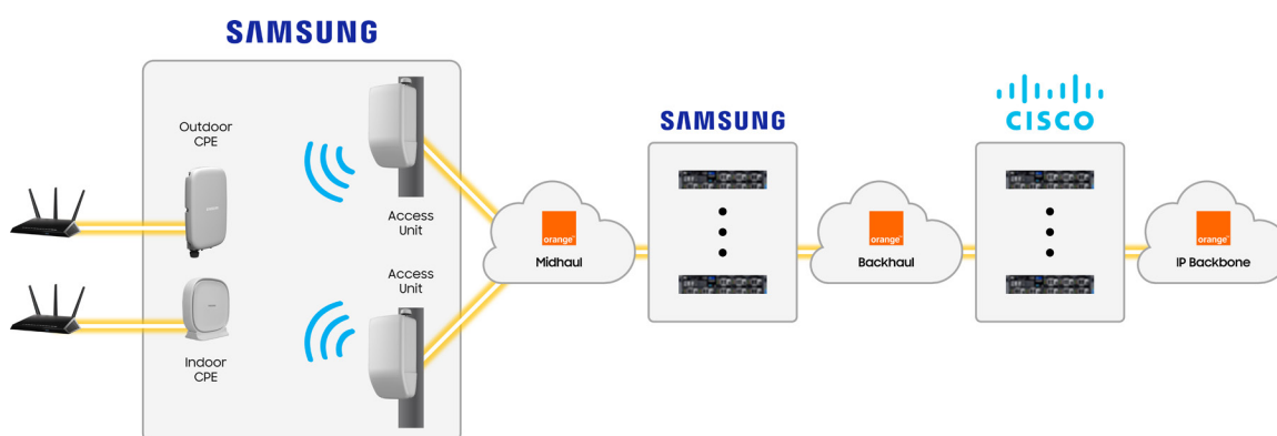
Figure 8 : Orange Romania 5G FWA Friendly User Trial Architecture
