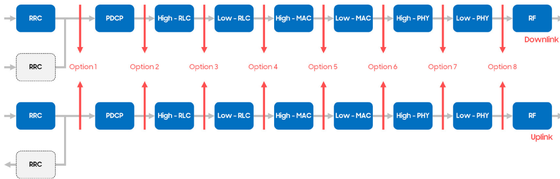
Figure 7 : Radio Access Functional Split
