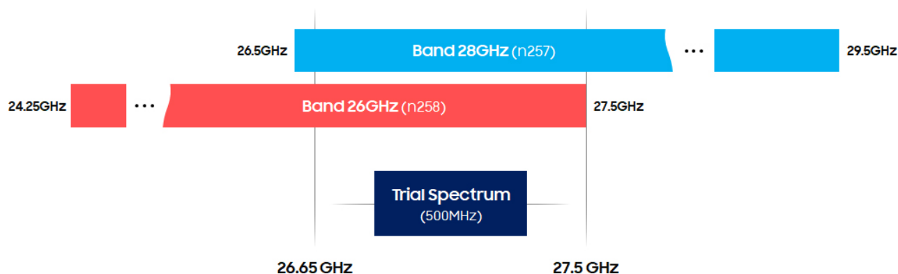
Figure 9 : Trial Spectrum
