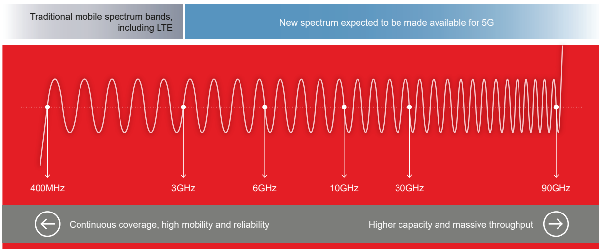
Figure 3: 5G spectrum
