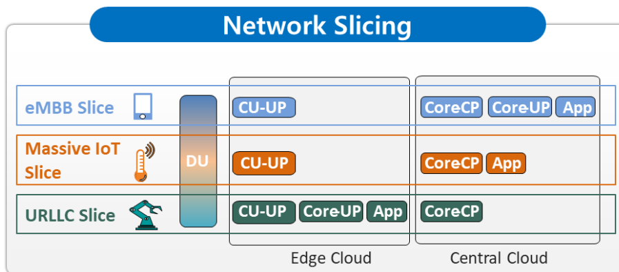
Figure 7. Examples utilizing network slicing
