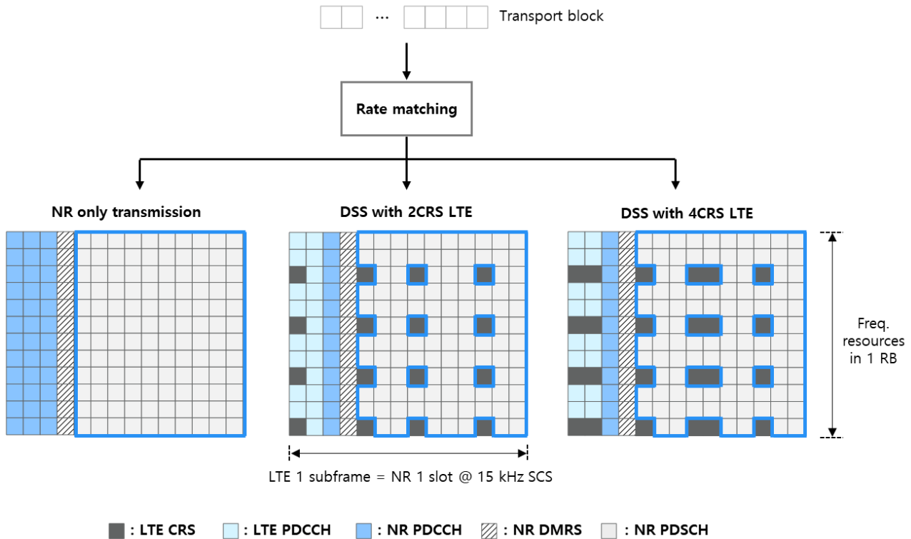
Figure 9. Examples of NR PDSCH with CRS rate matching
