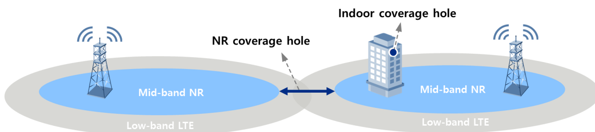
Figure 3. Coverage hole of mid-band NR
