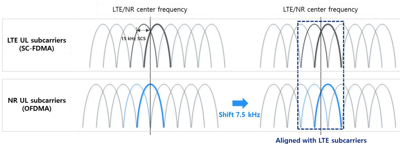
Figure 8. NR UL 7.5 kHz shift to align with LTE UL grid
