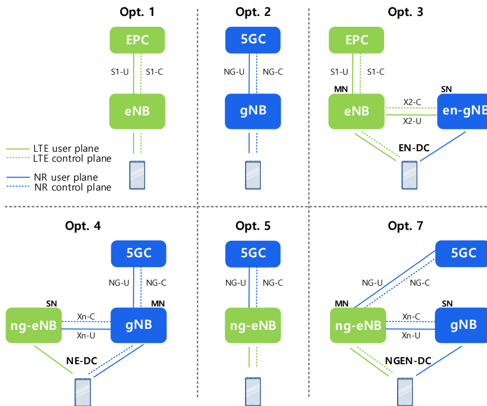
Figure 2. NR deployment architecture options
