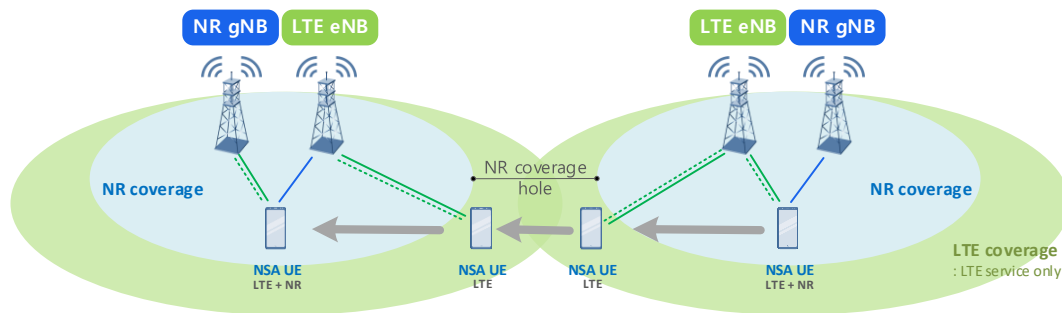
Figure 13. Mobility support with NSA option 3
