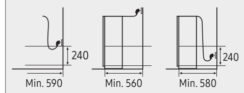
Minimum Cabinet Depth
