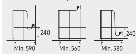
Minimum Cabinet Depth
