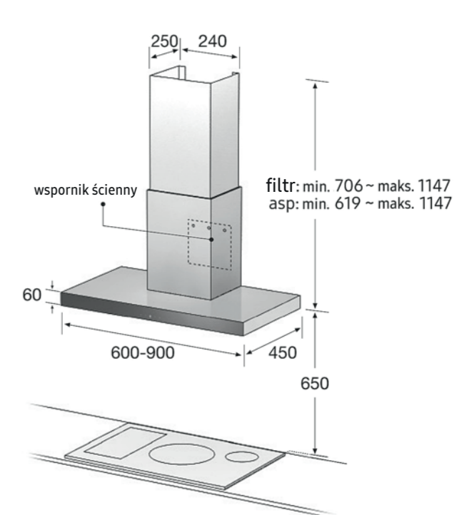
Rysunek techniczny dotyczy modeli: NK36M5070BS, NK24M5070BS, NK36M5060SS
